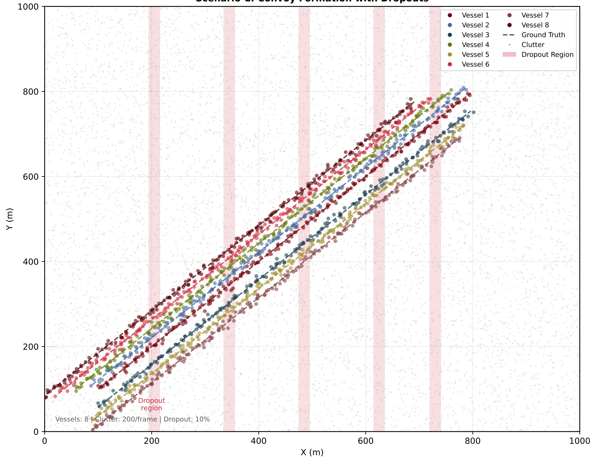
Scenario C: Convoy Formation with Dropouts
